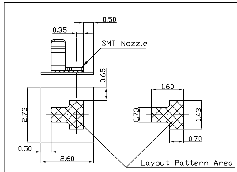
PCB Recommend Layout Pattern
